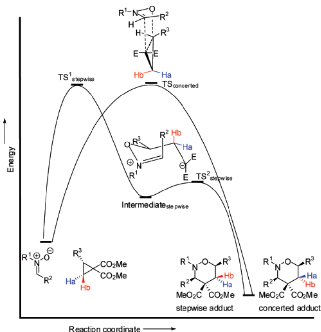
FIGURE 1. Stepwise and concerted mechanisms for cycloaddition.
