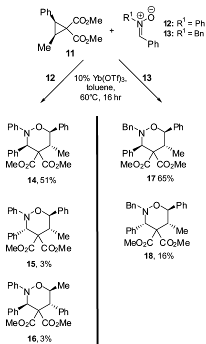
SCHEME 2. Reaction of Cyclopropane 11 with Nitrones 12 and 13
