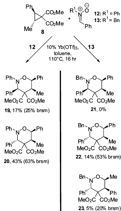
SCHEME 3. Reaction of Cyclopropane 8 with Nitrones 12 and 13
