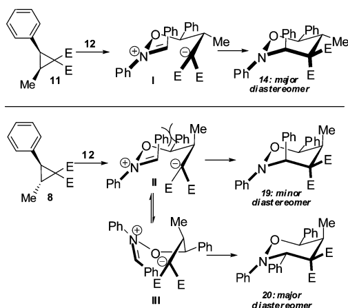
FIGURE 2. Mechanistic rationale for observed product mixture.
