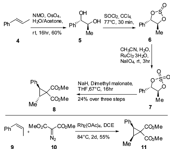
SCHEME 2. Reaction of Cyclopropane 11 with Nitrones 12 and 13
